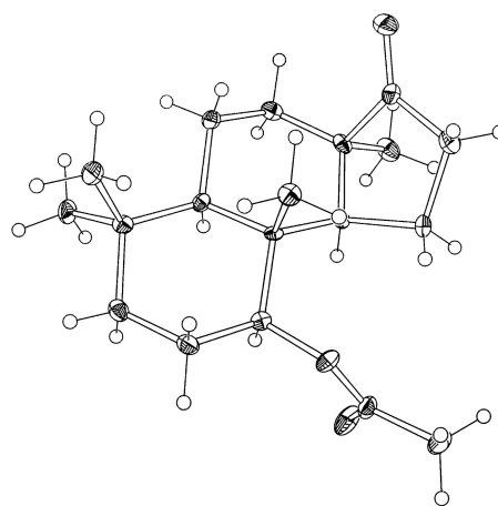
Figure 2. X-ray structure of ( \pm )-12.
