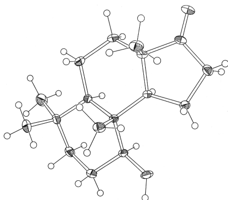
Figure 1. X-ray structure of ( \pm )-8c.
